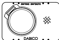
DAB-40WP PIT OPENING 1016 X 644 (COVER FRAME REMOVED) DOOR OPENING 457 \phi
