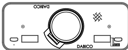
DAB-725/18WP PIT OPENING 1905 X 635 WITH 457 \phi CIRCULAR OPENING
