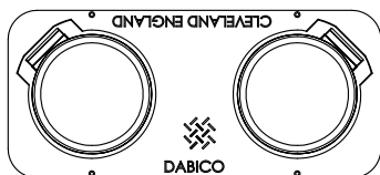
DAB-61WP PIT OPENING 1562 X 648 (COVER FRAME REMOVED) DOOR OPENING 457 \phi
