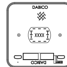
DAB-38WP PIT OPENING 965 X 965
